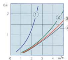
Head loss in service depending on drawing flow and adjustment.
