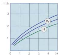
Washing (L) and rinsing (R) flow rates depending on water pressure.
